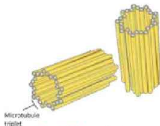
Figure 3.26: Two centrioles
