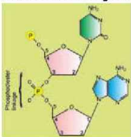
Figure 4.42: A dinucleotide
